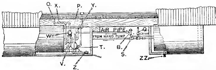
Fig. 3535. Part Sectional Elevation, showing Piping and Connections between Air-tank and Water-tank.
